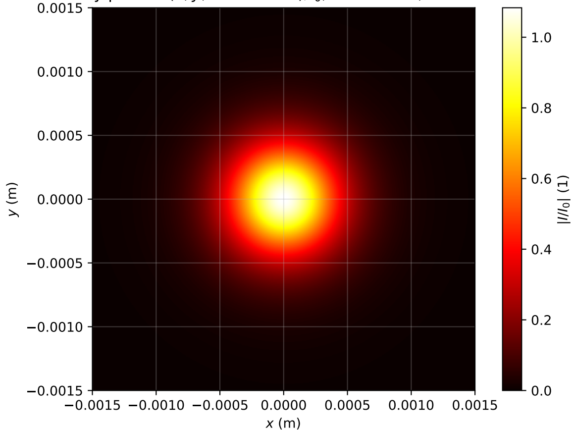
Intensity profile I(x, y, z = 2.070m)/I_0 , P_{in}=0.7P_{cr} , artificial time
